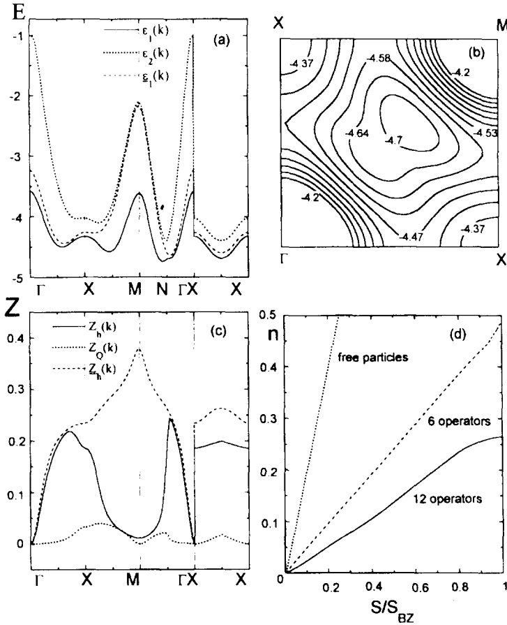
Fig.1. a) The spectra \varepsilon_1(\mathbf{k}) and \varepsilon_2(\mathbf{k}) calculated for the basis (2), (3), and the spectrum \underline{\varepsilon}_1(\mathbf{k}) calculated for the basis (2). The spectra are given along symmetrical lines \Gamma - X - M - N - \Gamma and X - N - X ; \Gamma = (0, 0) ; X = (\pi, 0), (0, \pi) , M = (\pi, \pi) ; N = (\pi/2, \pi/2) . b) Spectrum equal-energy lines \varepsilon_1(\mathbf{k}) = \text{const.} c) Z_h(\mathbf{k}) and Z_Q(\mathbf{k}) - the number of bare holes (the residues of corresponding Green's functions) in the quasiparticle excitations for the spectra \varepsilon_1(\mathbf{k}) and \underline{\varepsilon}_1(\mathbf{k}) ; Z_Q(\mathbf{k}) is the residue of the lowest pole \varepsilon_1(\mathbf{k}) ; for the Green's function G_{11,11}(\omega, \mathbf{k}) + G_{12,12}(\omega, \mathbf{k}) , which characterize the "shadow band" effect. d) the dependence of the number of holes n per unit cell on the value of the Fermi surface area S ( S_{BZ} - the area of the first Brillouine zone): thick line - for the spectrum \varepsilon_1(\mathbf{k}) ; dashed line - for the spectrum \underline{\varepsilon}_1(\mathbf{k}) ; solid straight line - the case of the noninteracting particle filling
