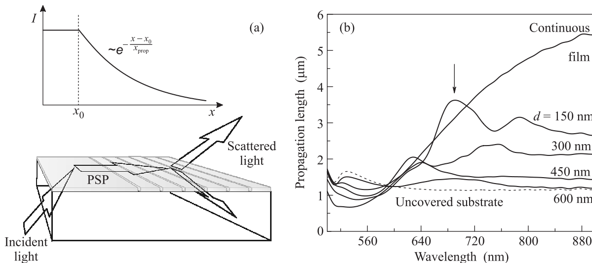
Fig. 5. (a) – Schematic representation of the modeled experiment provided to define the PSP propagation length x_{\text{prop}} . PSPs are excited by an incident wave on a smooth gold film using the Kretschmann prism-coupling configuration. The excitation region is to the left of x_0 . To the right of x_0 , the film is perforated with a period of 750 nm. The PSP amplitude A(x) decays exponentially because of radiative and ohmic losses. (b) – The spectral dependence of the PSP propagation length along the nanograting in the x direction. The slit width is varied in the range from 150 to 600 nm with a step of 150 nm; the grating period is set to 750 nm. The black curve shows the propagation length spectral dependence for the smooth film, and the olive curve shows the decay distance of the electromagnetic field at the edge of the gold film
