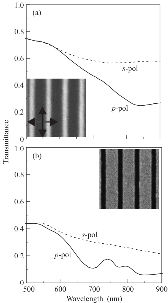
Fig. 1. Normal incidence transmittance spectra for nanogratings with slit widths of 500 nm (a) and 170 nm (b). Incident light is linearly polarized along the stripes (dashed curves) or perpendicular to them (solid curves). Insets show 3 \times 3 \mu\text{m}^2 SEM images of the samples; the corresponding light polarization orientation is indicated by arrows
