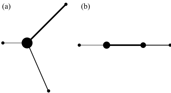
(a) Dressed three-bond star graph and (b) dressed four-vertex chain graph. Different potential strengths on the bonds are indicated by different thickness of the bonds. Different vertex strengths are indicated by different dot sizes representing the vertices
