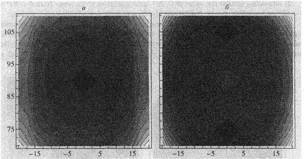
Fig.2. Energy minimum in the \phi - \theta -plane just before (left) and just after (right) the onset of tilted rotation. Note the local maximum developing at the centre. The example chosen is N = 36 , a tri-axial near oblate nucleus
