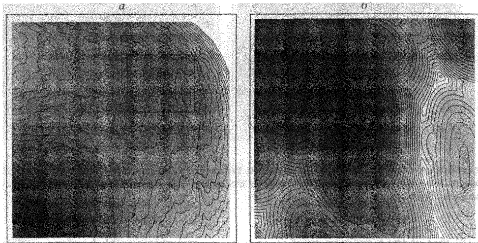
Fig.1. Energy contours in the \omega_x - \omega_y -plane for a rotational speed where the onset of an oblate shape has just taken place and corresponds to the local minimum shown in the right figure. However, for the nucleus considered ( N = 44 , tri-axial near prolate) a much deeper minimum has developed as an instability as seen in the top left corner of the left figure. The section of the top illustration is indicated in the bottom part
