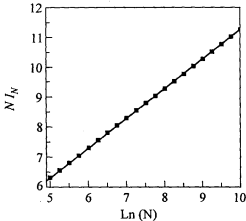
The polarisation energy of small Fröhlich polarons trapped in a string depends on its length as \ln N/N
