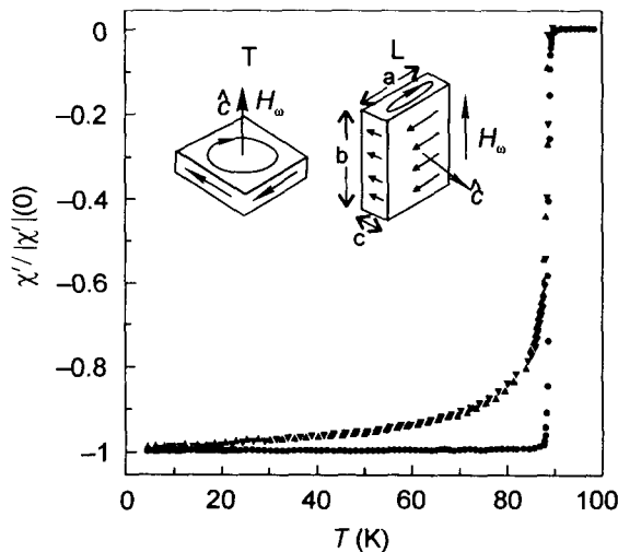
Fig.1. Curves of the ac -susceptibility of sample #1 versus temperature in different orientation with respect to ac magnetic field: H_\omega \parallel c (full circles); H_\omega \perp c , H_\omega is parallel to the b -edge of the crystal (up triangles); H_\omega \perp c , H_\omega is parallel to the a -edge of the crystal (down triangles). Left-hand inset: transverse (T) orientation, H_\omega \parallel c , the arrows on the surfaces show directions of the screening current. Right-hand inset: Longitudinal (L) orientation, H_\omega \perp c
