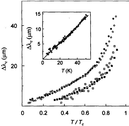
Fig.3. Temperature dependences \Delta\lambda_c in samples #1 (circles) and #2 (squares) at T < 0.9T_c . Open symbols plot low-frequency measurements, full symbols show microwave data. The inset shows low temperature sections of the \Delta\lambda_c curves in sample #1
