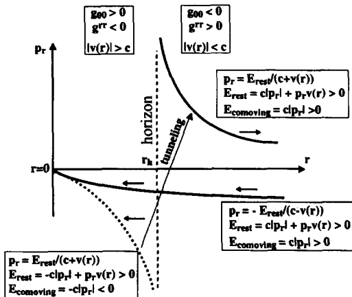
Fig.3. Tunneling from Minkowski vacuum within the horizon to the outgoing mode
