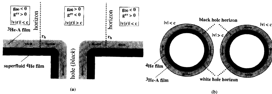
Fig.1. Simulation of 2D black hole in thin ^3\text{He-A} film. (a) Draining bathtub geometry. (b) ^3\text{He-A} film circulating on the top of the ^4\text{He} film on torus
