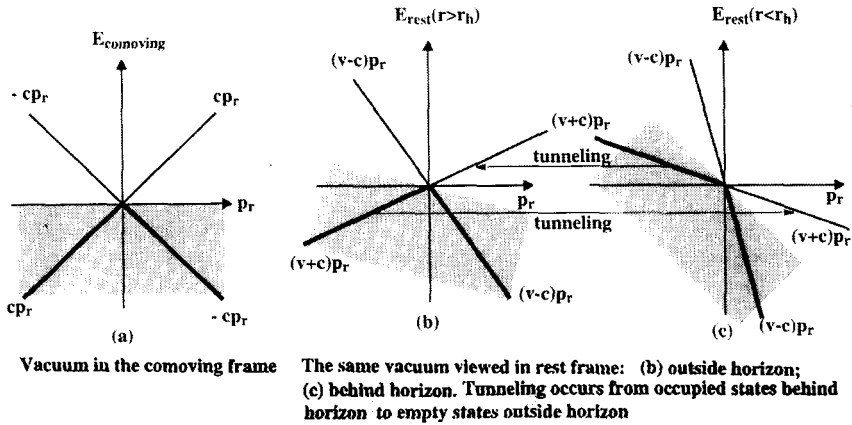
Fig.2. (a) Fermionic vacuum in the comoving frame. The states with E_{com} < 0 are occupied (thick lines). The same vacuum viewed in the rest frame (b) outside horizon and (c) inside horizon. Behind the horizon the branch E_{rest} = (v + c)p_r (for p_{\perp} = 0 ) has inverse population as seen in the rest frame: the states with positive energy E_{rest} > 0 are filled, while the states with E_{rest} < 0 are empty. The tunneling across horizon from the occupied states to the empty states with the same energy gives rise to the Hawking radiation from the horizon
