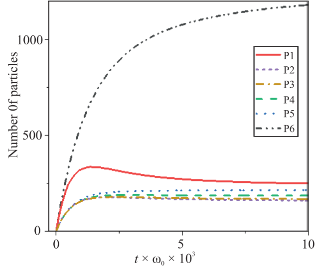
Fig. S1. Time dependence of the population of polariton modes at constant pumping \frac{I}{\omega_0} = 3.001 near zero
