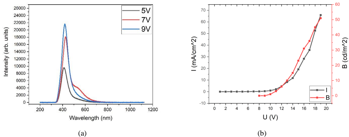
Fig. S1. (a) Electroluminescence spectrum of the OLED structure ITO/PEDOT-PSS(50 nm)/poly-TPD(20 nm)/CA-2-CDs/TPBi(15 nm)/LiF(1 nm)/Al(50 nm). The additional bend in the band at 630 nm observed at 7 V is presumably attributed to electroluminescence from the transport layers, poly-TPD and/or TPBi, (b) I-V curve and brightness-voltage dependence of the OLED structure.
