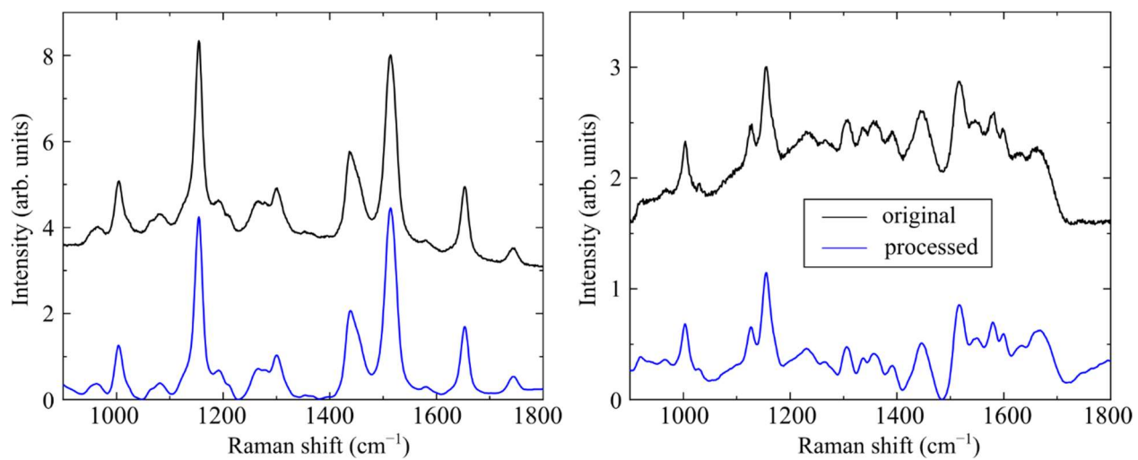
Fig. S1. Examples of original spectra (black) and spectra after baseline subtraction and smoothing (blue)
